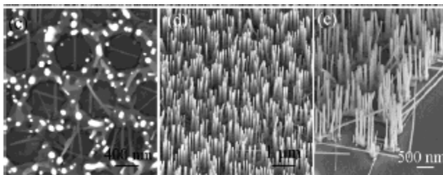
Figure 5: Top and 30° view of aligned ZnO nanorods, where the hexagonal pattern is apparent: (d) aligned ZnO nanorods at the edge of the growth pattern
